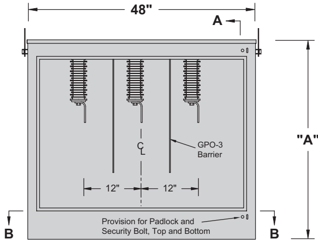
Front View Door & Door Safety Barrier Removed
