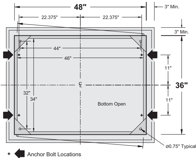
Section BB with Typical Pad Dimensions
