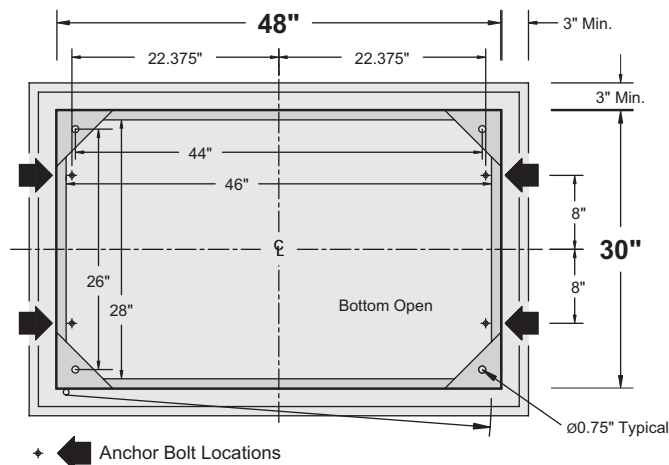
Section BB with Typical Pad Dimensions
